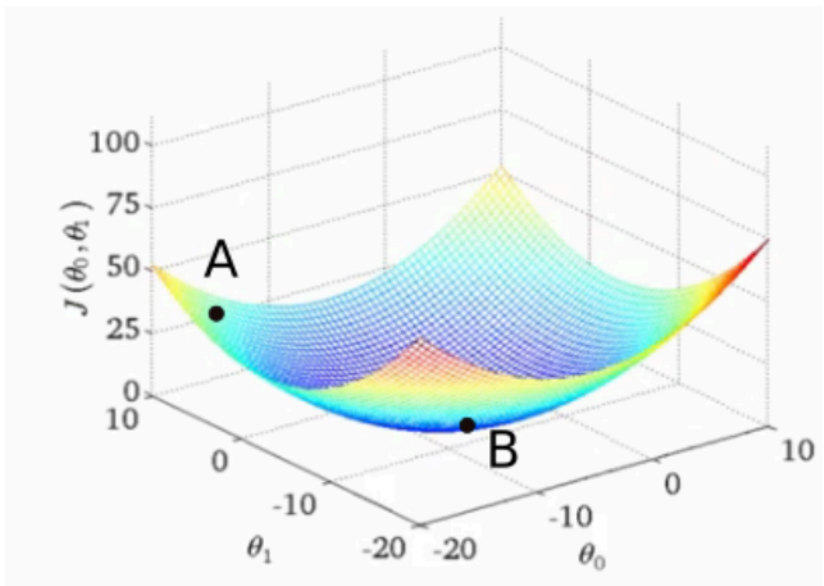
Fig. 5: Gradient Descent
