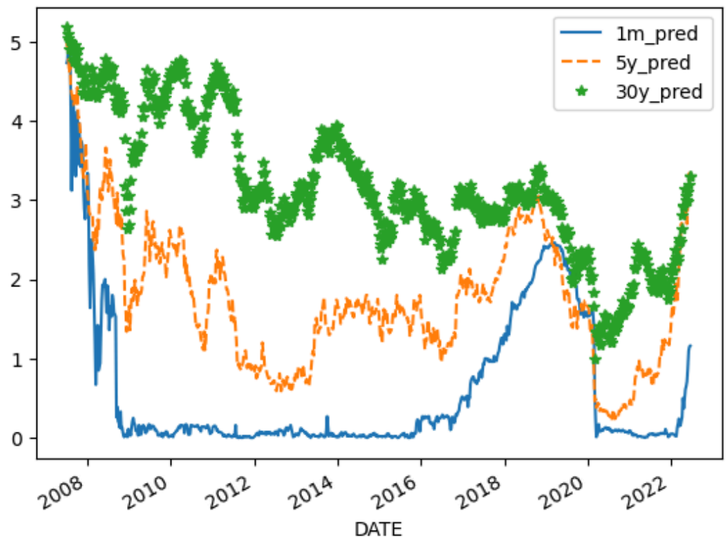
Fig. 5: Yield Curve Prediction
