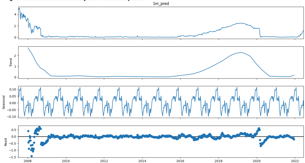
Fig. 8: Time Series Trend Analysis for 1 month period
