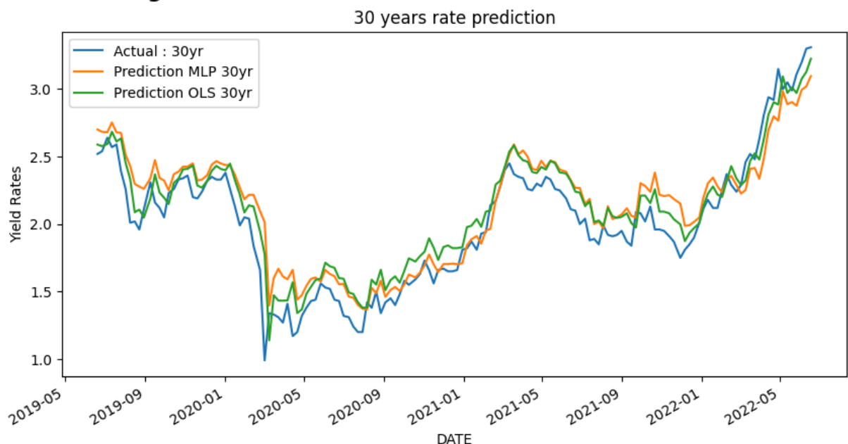
Fig. 18: 30 Year Prediction
