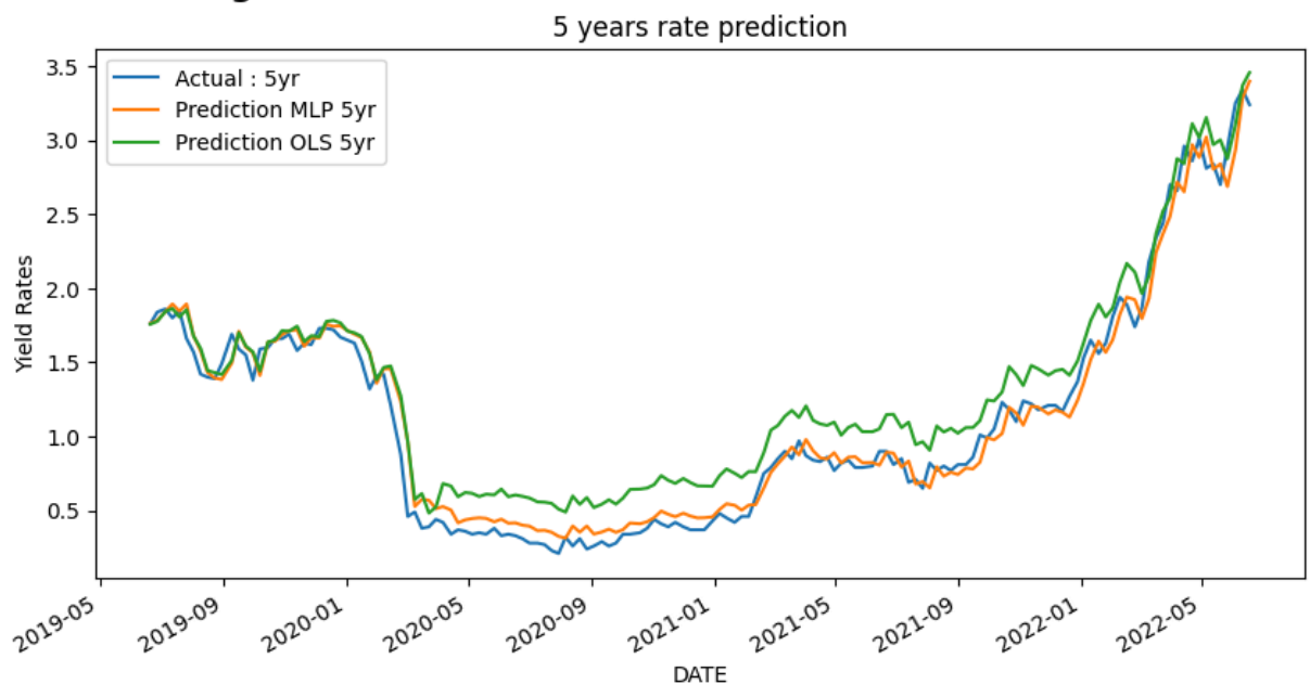
Fig. 17: 5 Years Prediction
