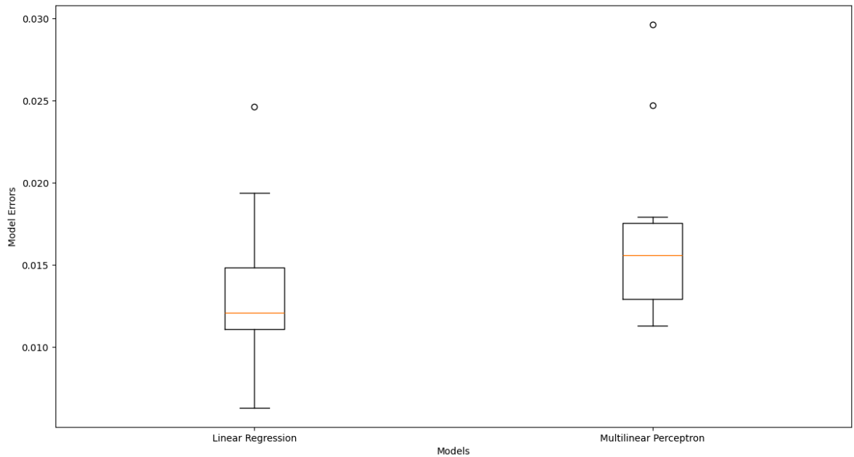
Fig. 14: Box Plot Comparing Model Performance
