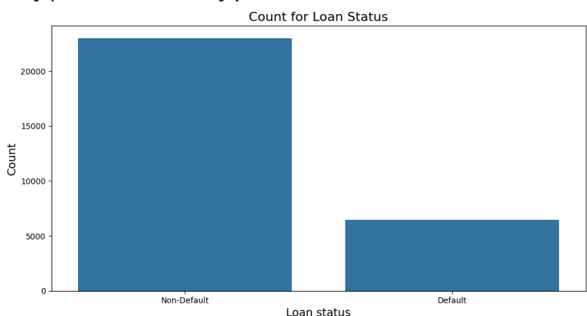
Fig. 1: Top: A bar plot of good versus bad loans. The graph shows that the dataset is highly imbalanced.
